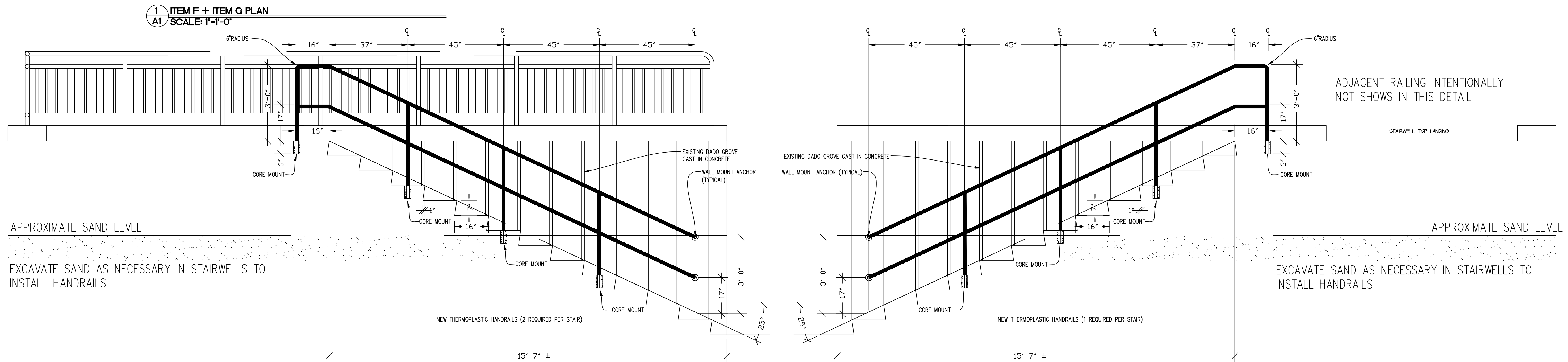
2 ITEM F HANDRAIL DETAIL AT SECTION THRU STAIRWELLS 1-4 NORTH OF MARINE MEMORIAL (TYPICAL) A1 SCALE: 1/4"=1'-0"
